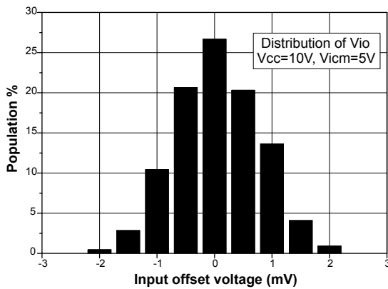
Figure 4. Distribution of input offset voltage at V_{\text{CC}} = 10 \text{ V}
