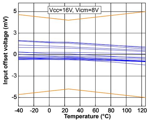
Figure 6. Input offset voltage vs. temperature at V_{\text{CC}} = 16 \text{ V}
