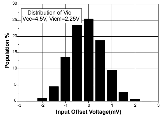
Figure 3. Distribution of input offset voltage at V_{\text{CC}} = 4.5 \text{ V}
