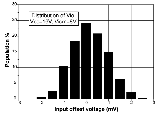
Figure 5. Distribution of input offset voltage at V_{\text{CC}} = 16 \text{ V}
