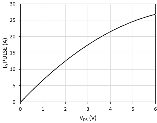
Fig. 2. Pulsed Drain current ( I_D PULSE) vs. drain-to-source voltage ( V_{DS} ) at T = 25^\circ\text{C}
