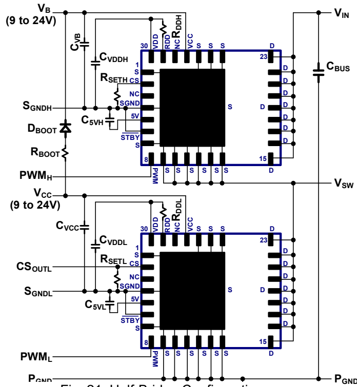
Fig. 21. Half-Bridge Configuration
