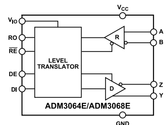
Figure 4. ADM3064E/ADM3068E Functional Block Diagram
