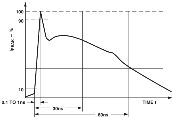
Figure 11. IEC1000-4-2 ESD Current Waveform
