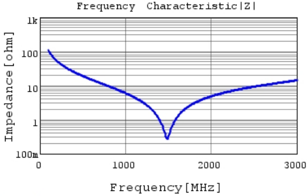
GRM31A7U3A150JW31 |Z| DC0V, 25degC
