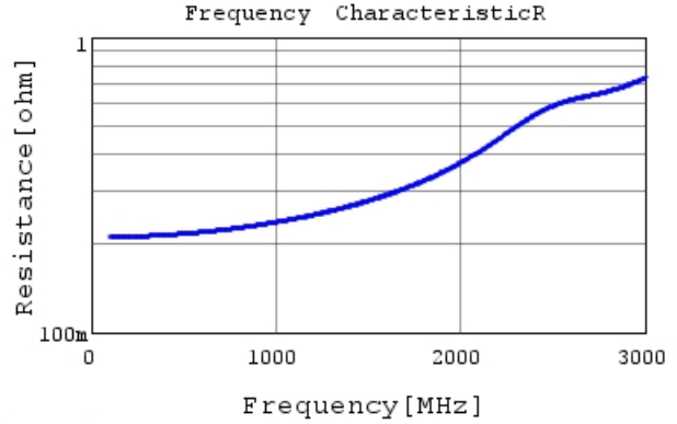
GRM31A7U3A150JW31 R DC0V, 25degC
