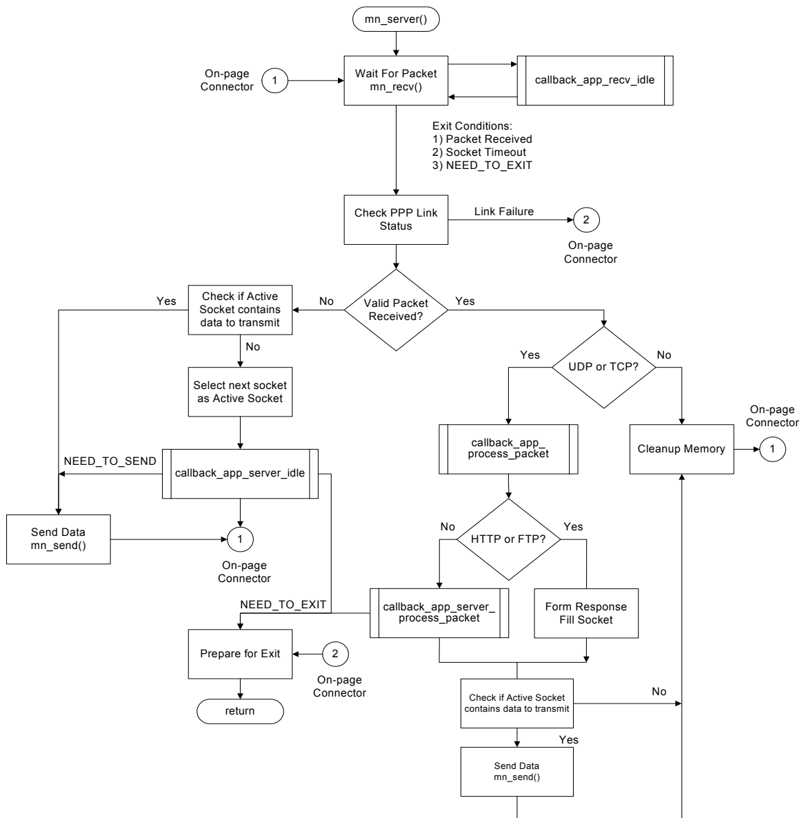
Figure 2. Callback Function Flow Diagram
