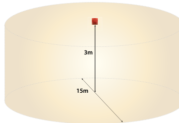
EN54-23 Coverage: C-3-15
