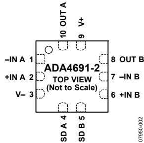
Figure 4. 10-Lead, 2 mm × 2 mm LFCSP (CP-10-11)
