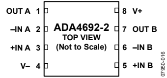
Figure 6. 8-Lead, 2 mm × 2 mm LFCSP (CP-8-6)
