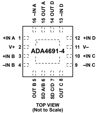
NOTES 1. IT IS RECOMMENDED THAT THE EXPOSED PAD BE CONNECTED TO V-. Figure 5. 16-Lead, 3 mm × 3 mm LFCSP (CP-16-22)
