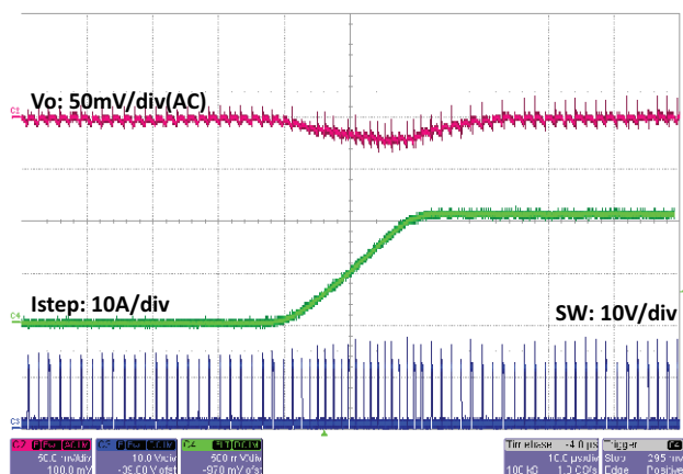
Fig. 55 - SiC450 Load Step, 0 A to 20 A, 1 A/µs, t = 10 µs/div
