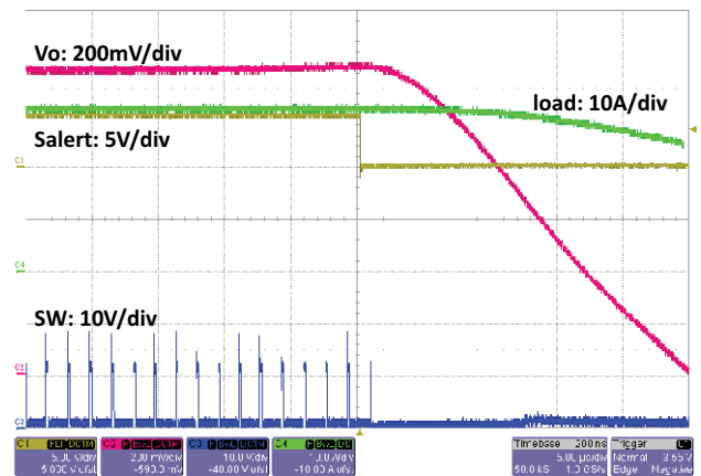
Fig. 33 - SiC451 OCP
