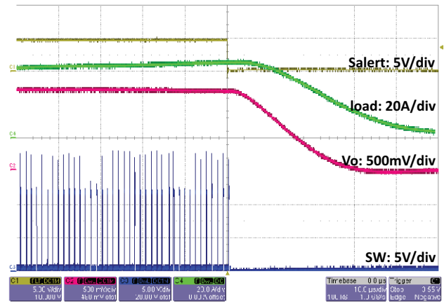
Fig. 51 - SiC450 Overcurrent Protection Behavior, t = 10\text{ }\mu\text{s}
