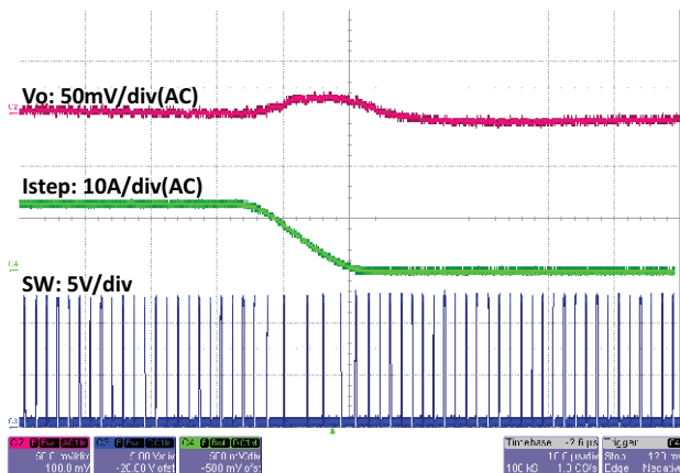
Fig. 36 - SiC451 Load Step, 25 A to 12.5 A, 1 A/ \mu\text{s} , t = 10\text{ }\mu\text{s/div}
