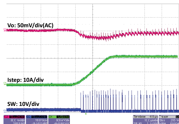
Fig. 57 - SiC450 Load Step, 0 A to 20 A, 1 A/µs, t = 10 µs/div Skip Mode Enabled
