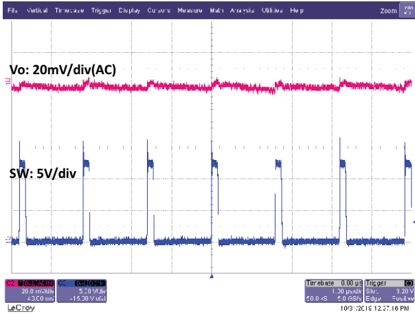
Fig. 59 - SiC450 Output Ripple, 0.01 A, t = 1\text{ }\mu\text{s/div} Forced Continuous Conduction Mode
