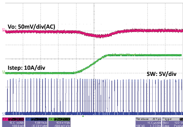
Fig. 37 - SiC451 Load Step, 0 A to 12.5 A, 1 A/ \mu\text{s} , t = 10\text{ }\mu\text{s/div}
