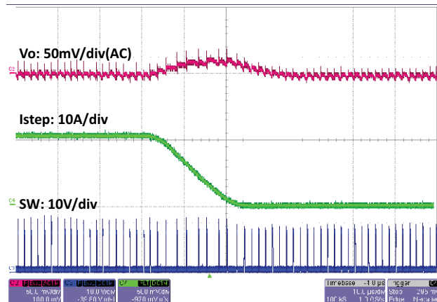
Fig. 56 - SiC450 Load Step, 20 A to 0 A, 1 A/µs, t = 10 µs/div
