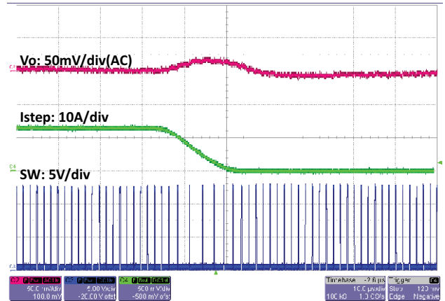
Fig. 38 - SiC451 Load Step, 12.5 A to 0 A, 1 A/ \mu\text{s} , t = 10\text{ }\mu\text{s/div}
