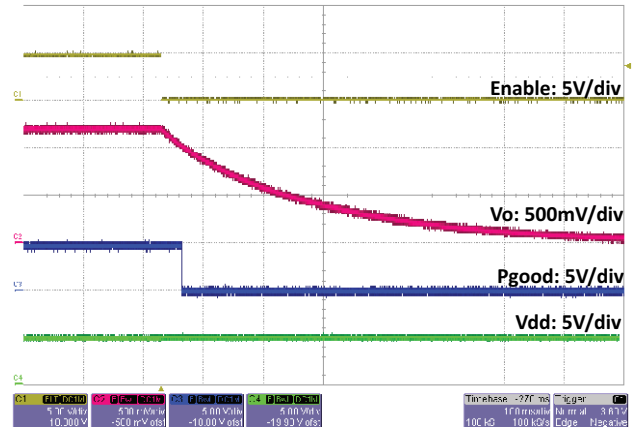
Fig. 32 - SiC451 Shut down with EN, t = 100\text{ ns/div}
