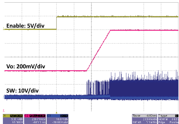
Fig. 45 - SiC451 Prebias Startup
