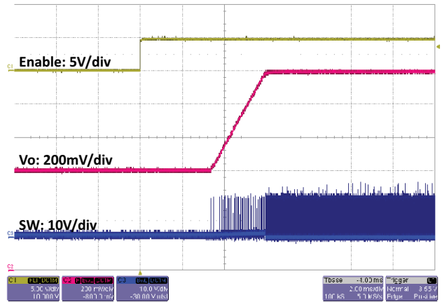
Fig. 63 - SiC450 Prebias Startup
