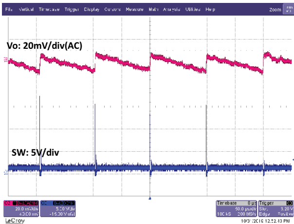
Fig. 60 - SiC450 Output Ripple, 0.01 A, t = 50\text{ }\mu\text{s/div} DCM Mode
