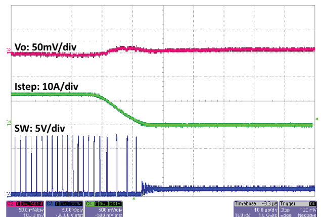
Fig. 40 - SiC451 Load Step, 12.5 A to 0 A, 1 A/ \mu\text{s} , t = 10\text{ }\mu\text{s/div} Skip Mode Enabled
