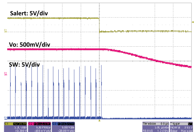
Fig. 52 - SiC450 Output Undervoltage Protection Behavior, t = 5\text{ }\mu\text{s/div}
