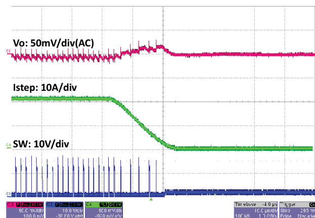
Fig. 58 - SiC450 Load Step, 20 A to 0 A, 1 A/µs, t = 10 µs/div Skip Mode Enabled
