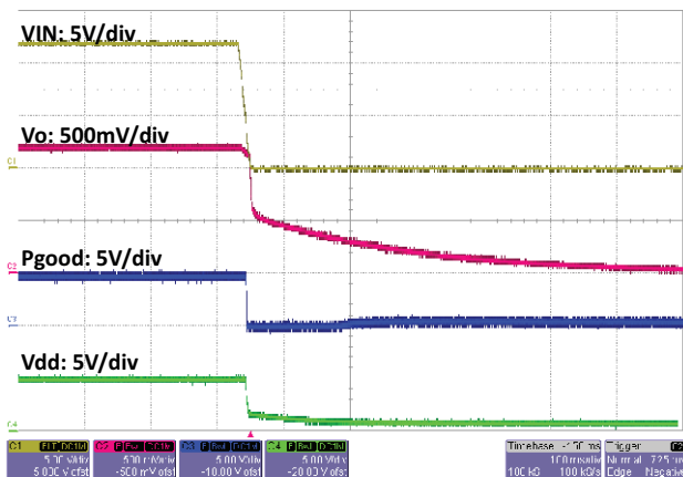
Fig. 30 - SiC451 Shut Down with V_{IN} , t = 100\text{ ns/div}
