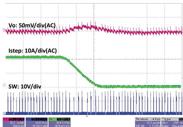
Fig. 54 - SiC450 Load Step, 40 A to 20 A, 10 A/µs, t = 10 µs/div
