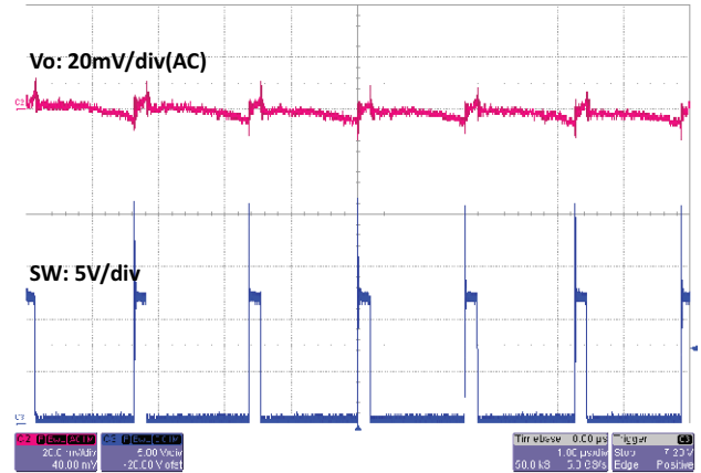
Fig. 44 - SiC451 Output Ripple, 25 A, t = 1\text{ }\mu\text{s/div} Forced Continuous Conduction Mode
