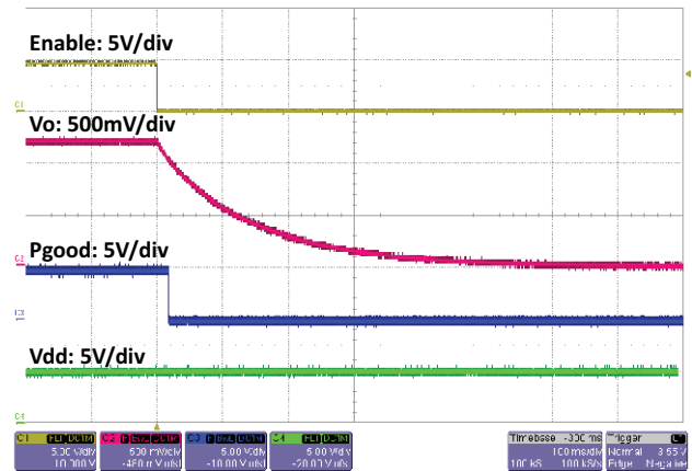
Fig. 50 - SiC450 Shut down with EN , t = 100\text{ ms/div}
