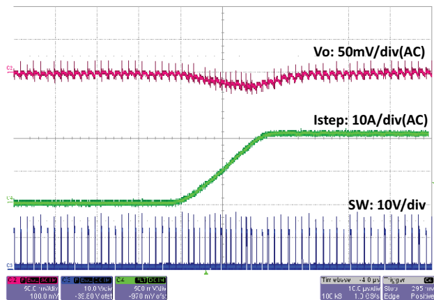
Fig. 53 - SiC450 Load Step, 20 A to 40 A, 1 A/µs, t = 10 µs/div
