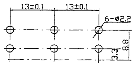
Dimensions of PC board holes (Commend)
