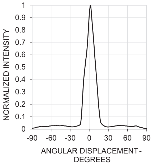
Figure 5: Radiation Pattern
