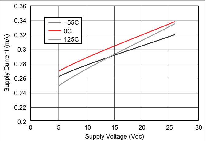
Figure 6-40. Supply Current vs Supply Voltage
