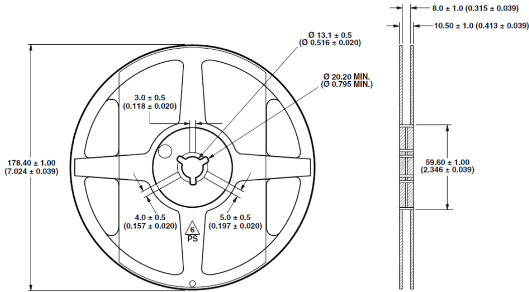
Figure 13: Reel Dimensions
