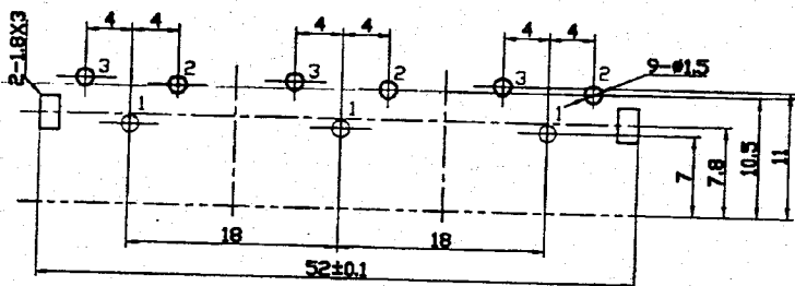
Dimensions of PC board hole (commend) (Top View) ⊗
