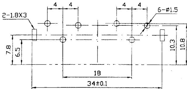
Dimensions of PC board hole
