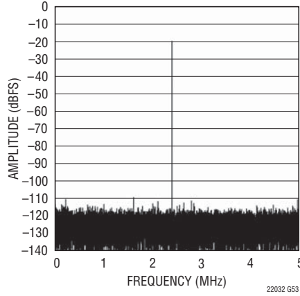
LTC2202: 32K Point FFT, f IN = 12.4MHz, -20dBFS, PGA = 0
