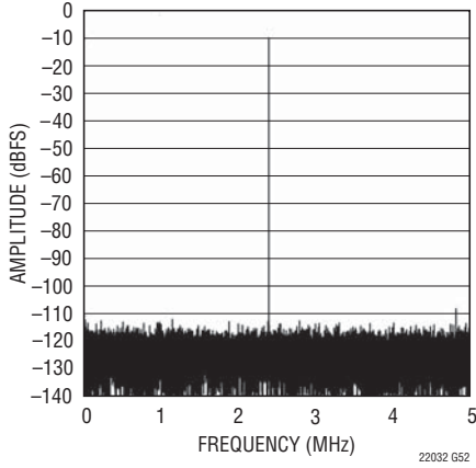
LTC2202: 32K Point FFT, f IN = 12.4MHz, -10dBFS, PGA = 0
