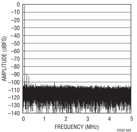
LTC2202: 32K Point FFT, f IN = 70.1MHz, -1dBFS, PGA = 1
