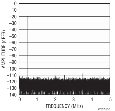
LTC2202: 32K Point FFT, f IN = 30.5MHz, -20dBFS, PGA = 1
