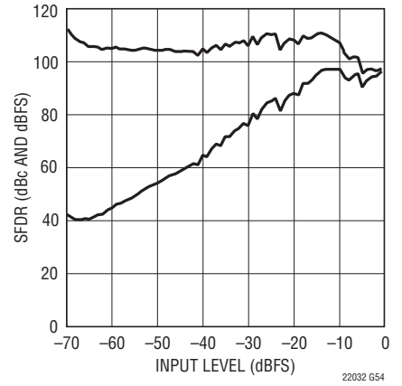
LTC2202: SFDR vs Input Level, f IN = 12.4MHz, PGA = 0, Dither "Off"
