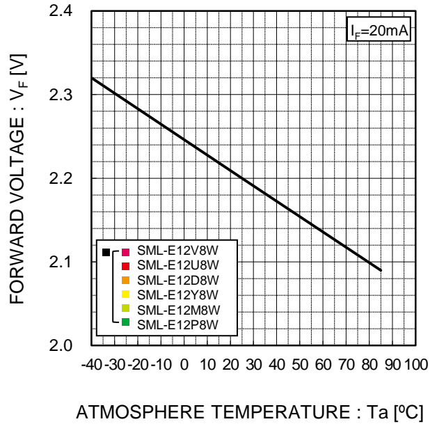
Fig.2 Forward Voltage - Atmosphere Temperature
