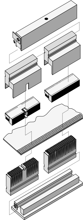
Modular press-fit tool for female connector modules 5+2
