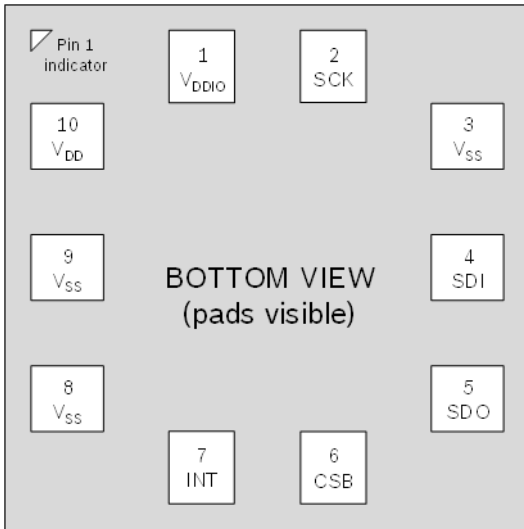
Pin configuration
