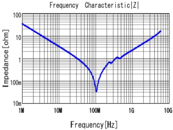
GCM2165C1H472JA16 |Z| DCOV, 25degC
