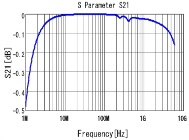
■ GCM2165C1H472JA16 S21 DCOV, 25degC
