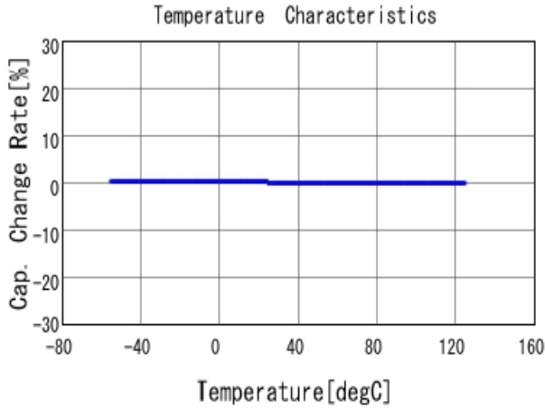
■ GCM2165C1H472JA16 C-Temp. capchange, DCOV, AC1Vrms
