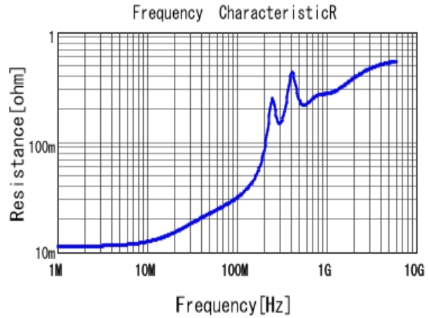
GCM2165C1H472JA16 R DCOV, 25degC
