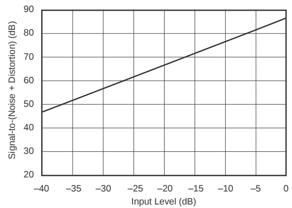
Figure 16. Signal-to-(Noise + Distortion) vs Input Level
