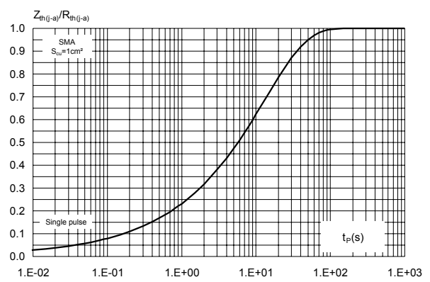
Figure 4. Relative variation of thermal impedance junction to lead versus pulse duration (SMA)
