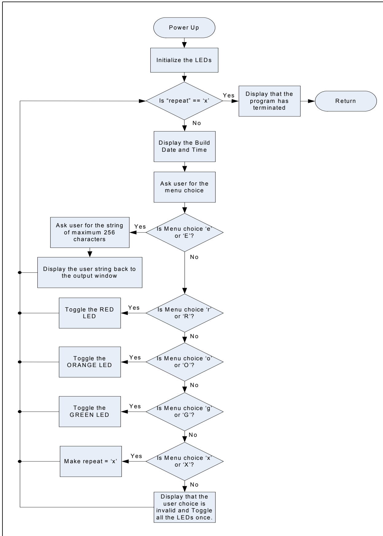
FIGURE 2-12: PIC32MX TUTORIAL PROGRAM FLOWCHART
