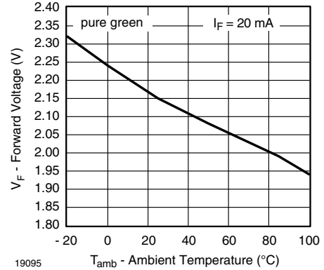
Fig. 16 - Forward Voltage vs. Ambient Temperature
