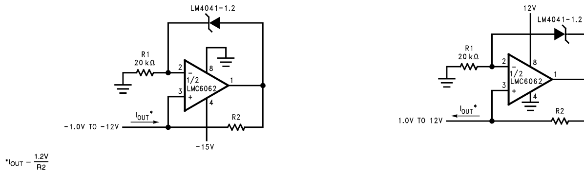
Figure 32. Precision 1 μA to 1 mA Current Sources
