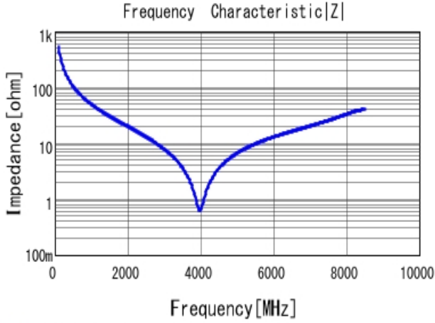
■ GRM1885C1H3R0CA01 |Z| DCOV, 25degC
