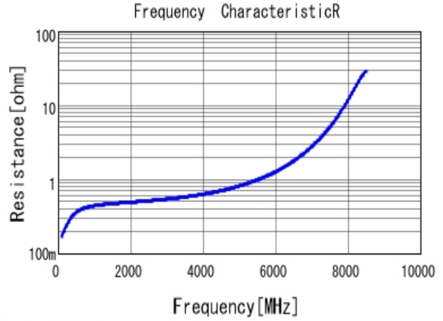
■ GRM1885C1H3R0CA01 R DCOV, 25degC
