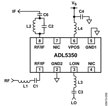
Figure 58. Reference Schematic
