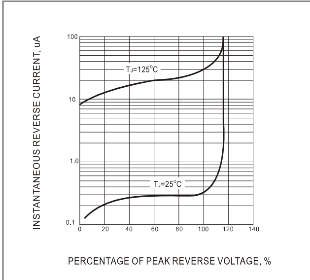
Fig.4 TYPICAL REVERSE CHARACTEISTICS
