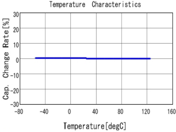
■ GRM3195C1H123JA01 C-Temp. capchange, DCOV, AC1Vrms
