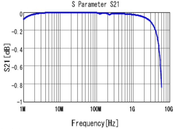
■ GRM3195C1H123JA01 S21 DCOV, 25degC
