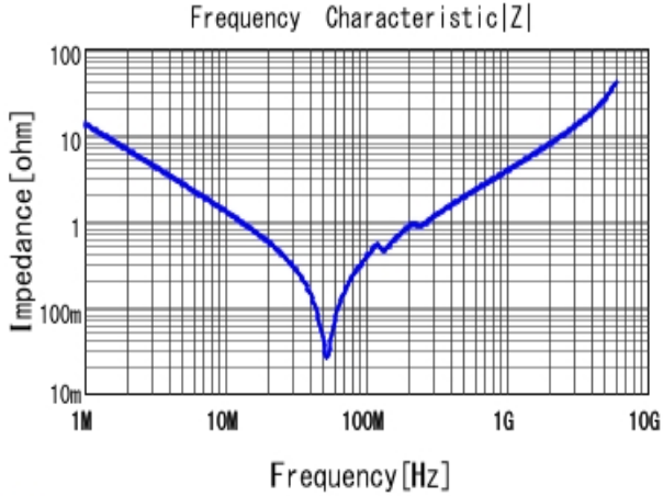
■ GRM3195C1H123JA01 |Z| DCOV, 25degC
