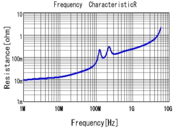
■ GRM3195C1H123JA01 R DCOV, 25degC
