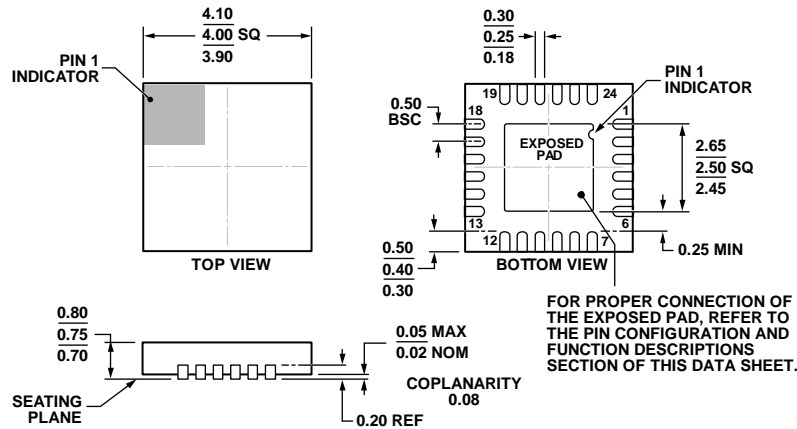
Figure 81. 24-Lead Lead Frame Chip Scale Package [LFCSP_WQ] 4 mm x 4 mm Body, Very Very Thin Quad (CP-24-7) Dimensions shown in millimeters
