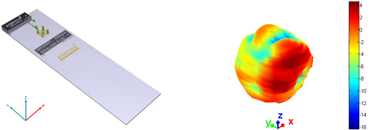
3D pattern at 2600MHz
