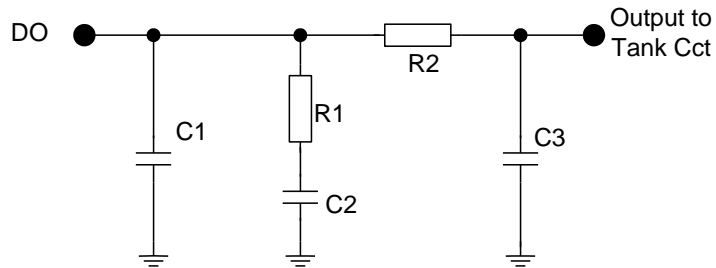
Figure 6 Example External Components – PLL Loop Filter
