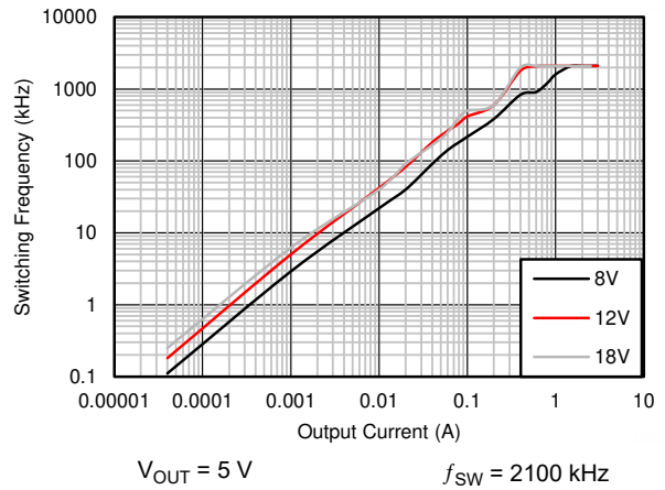
图 8-14. Switching Frequency versus Output Current
