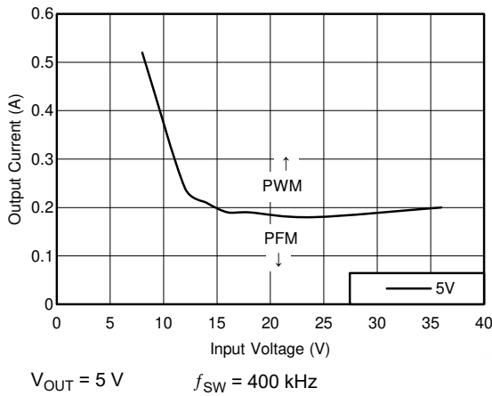
图 8-13. Mode Change Thresholds
