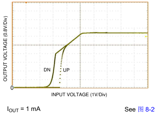
图 6-5. UVLO Thresholds
