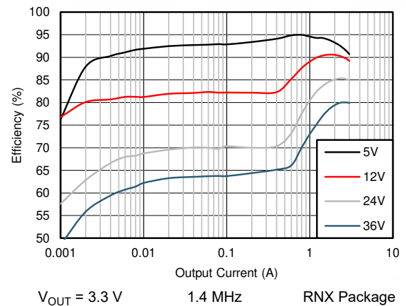
图 8-8. Efficiency
