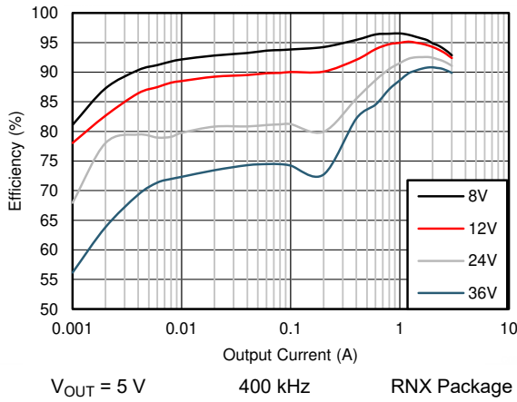
图 8-5. Efficiency
