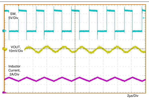
图 7-8. Typical PWM Switching Waveforms V_{IN} = 12 V, V_{OUT} = 5 V, I_{OUT} = 3 A, f_S = 400 kHz
