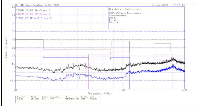
图 35. Radiated EMI Rod vs. CISPR25 Limits
