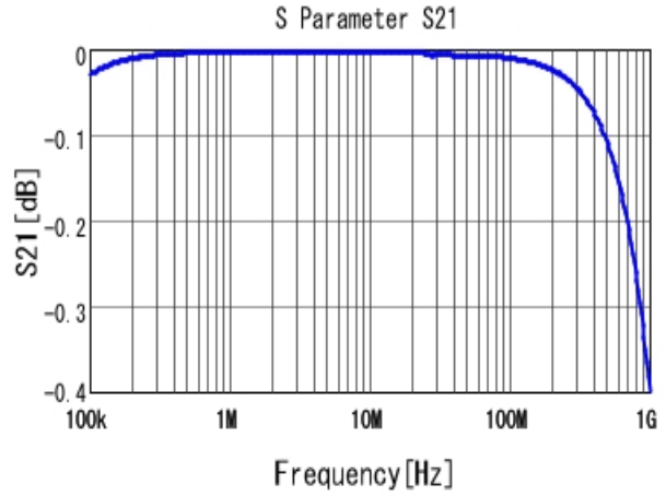
■ RDER71H224K1S1H03A S21 DC0V, 25degC
