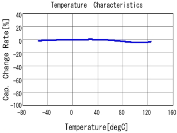
■ RDER71H224K1S1H03A C-Temp. capchange, DC0.0V, AC1.0Vr
