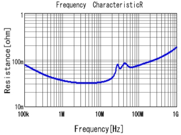
■ RDER71H224K1S1H03A R DC0V, 25degC
