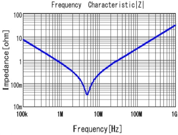
■ RDER71H224K1S1H03A |Z| DC0V, 25degC
