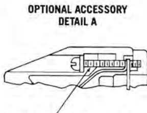
Captive Screw Kit (male) to be used with the Screw Lock Kit (female) for permanent secured fastening. Must be ordered separately. Part Number D111396. (Order 1 kit per connector.)
