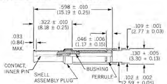
RECEPTACLE: DDMA110336 — RG196A/U and RG173B/U cable
