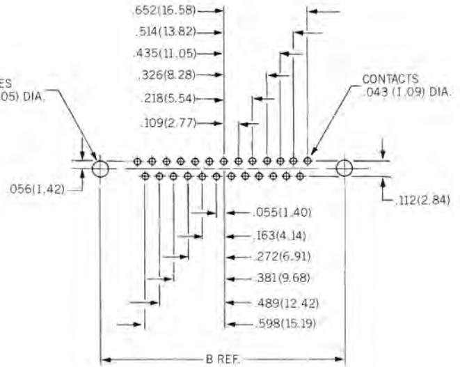
25 POSITION PCB HOLE PATTERN
