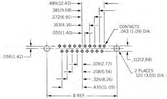
19 POSITION PCB HOLE PATTERN
