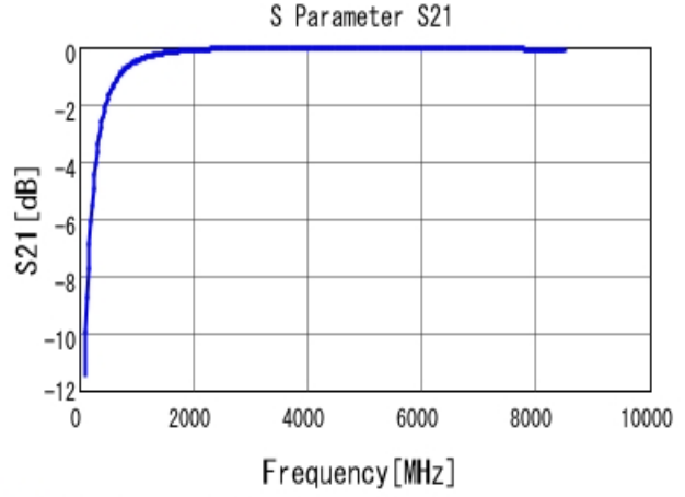
■ GJM0335C1E4R4BB01 S21 DCOV, 25degC
