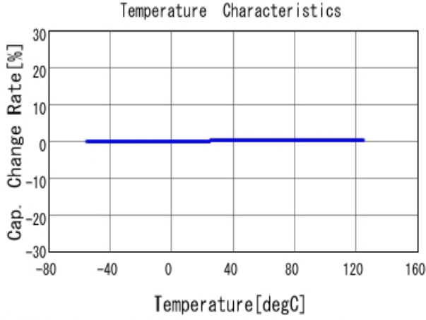
■ GJM0335C1E4R4BB01 C-Temp. capchange, DCOV, AC1Vrms
