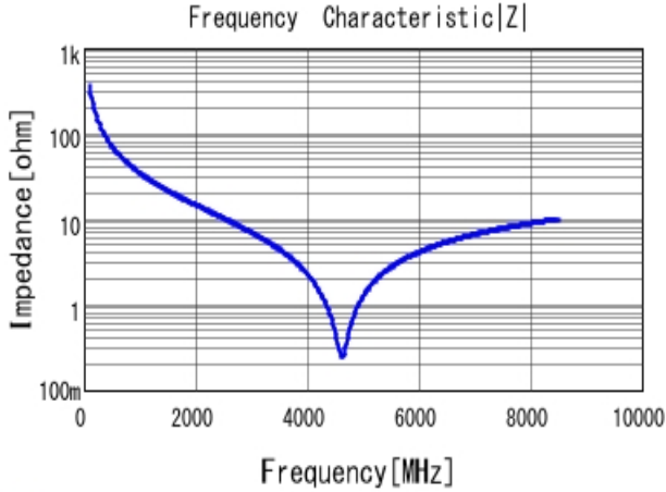
GJM0335C1E4R4BB01 |Z| DC0V, 25degC
