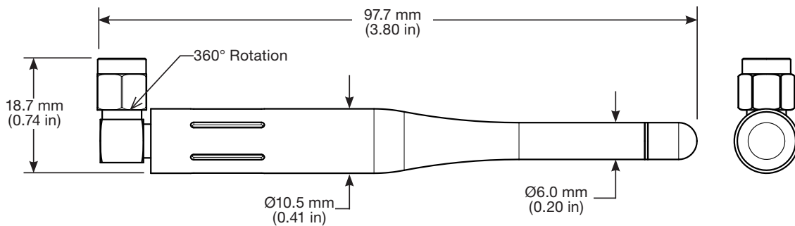
Figure 1. ANT-916-CW-RCL Antenna Dimensions
