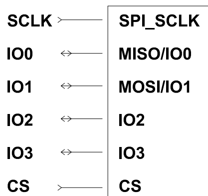
Figure 5. QSPI interface connection
