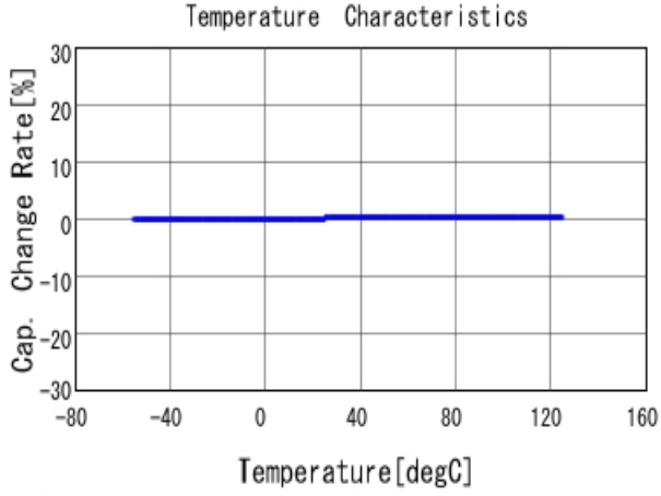
■ GJM0335C1E6R2CB01 C-Temp. capchange, DCOV, AC1Vrms
