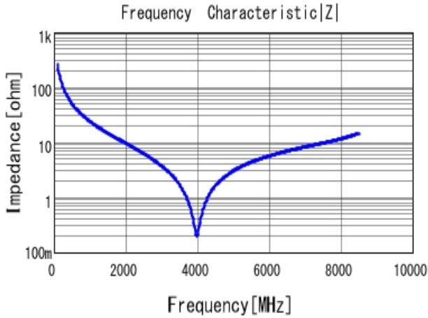
GJM0335C1E6R2CB01 |Z| DC0V, 25degC
