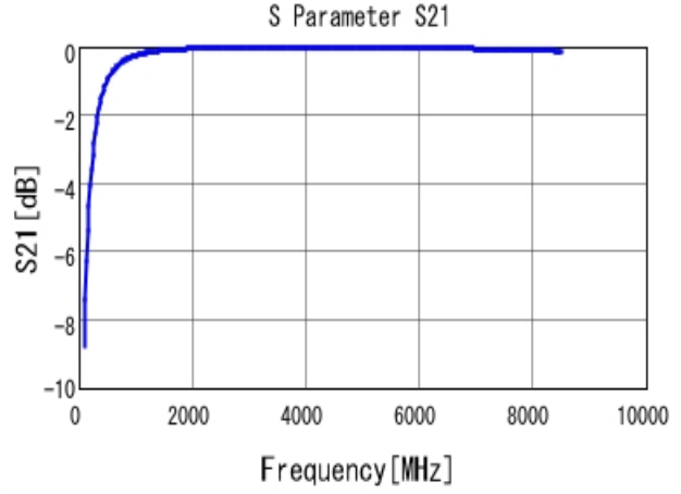
■ GJM0335C1E6R2CB01 S21 DCOV, 25degC
