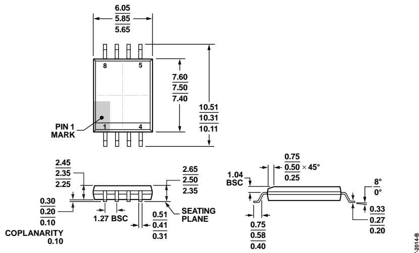
Figure 24. 8-Lead Standard Small Outline Package, with Increased Creepage [SOIC_IC] Wide Body (RI-8-1) Dimensions shown in millimeters
