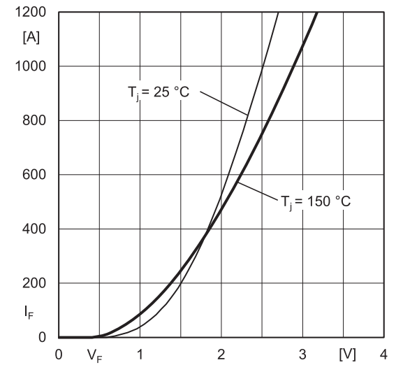
Fig. 10: Typ. CAL diode forward charact., incl. R_{CC+EE}
