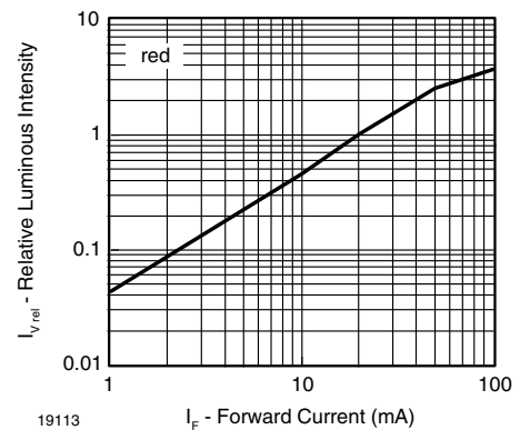
Fig. 26 - Relative Luminous Intensity vs. Forward Current
