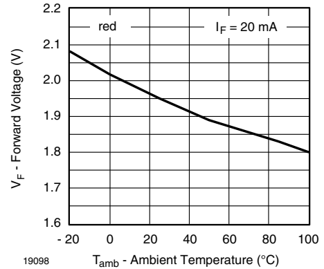
Fig. 24 - Forward Voltage vs. Ambient Temperature
