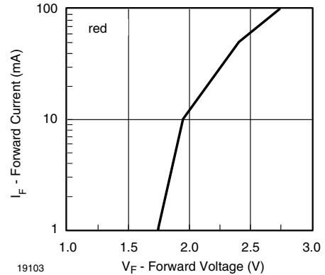
Fig. 25 - Forward Current vs. Forward Voltage
