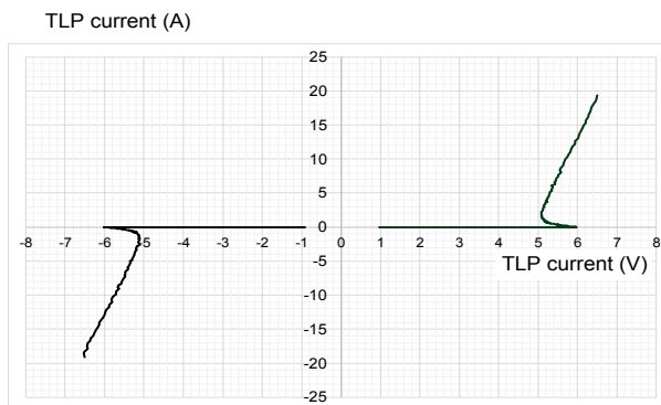
Figure 6. TLP characteristic
