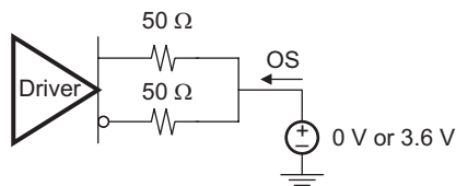
Figure 16. TMD5 Main Link Short-Circuit Output Circuit
