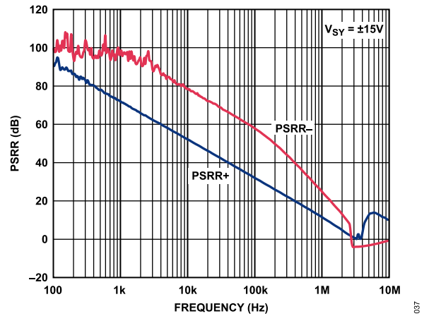
Figure 38. PSRR vs. Frequency, V_{SY} = \pm 15 V
