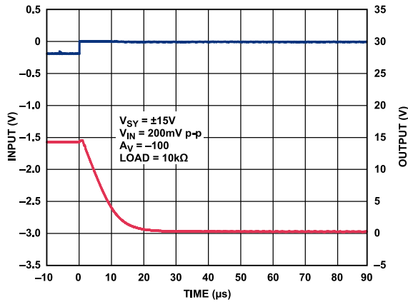
Figure 50. Positive Overload Recovery, V_{SY} = \pm 15\text{ V}
