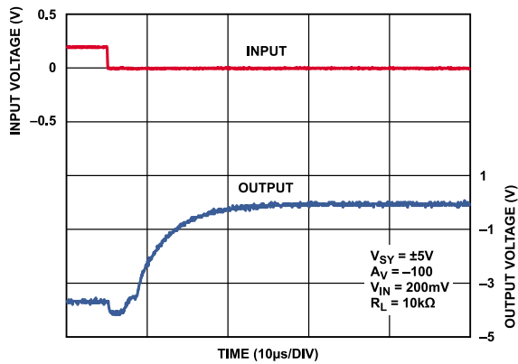
Figure 48. Negative Overload Recovery, V_{SY} = \pm 5\text{ V}
