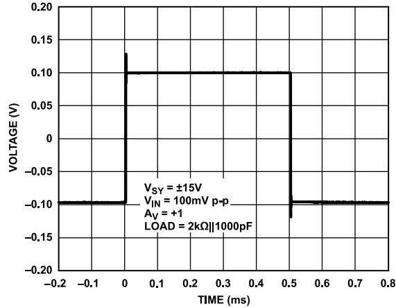
Figure 49. Small Signal Transient Response, V_{SY} = \pm 15\text{ V}
