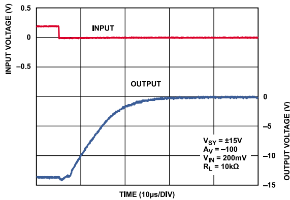
Figure 51. Negative Overload Recovery, V_{SY} = \pm 15\text{ V}
