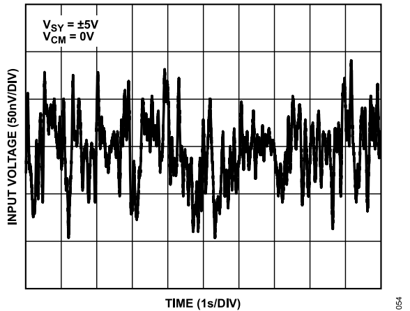
Figure 60. 0.1 Hz to 10 Hz Noise, V_{SY} = \pm 5\text{ V}
