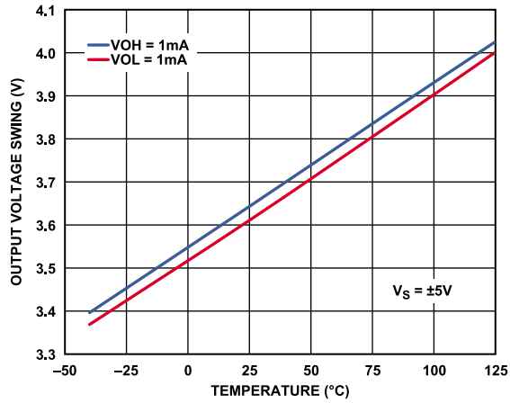
Figure 22. Output Voltage Swing vs. Temperature, V_{SY} = \pm 5 V
