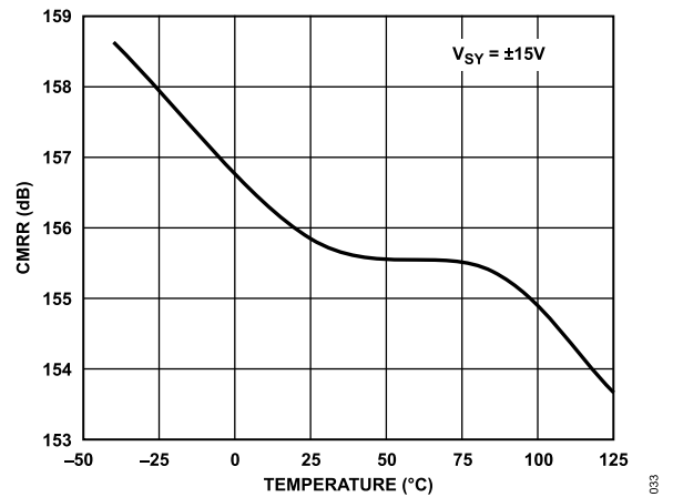
Figure 39. CMRR vs. Temperature, V_{SY} = \pm 15 V
