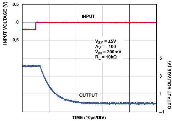
Figure 47. Positive Overload Recovery, V_{SY} = \pm 5\text{ V}
