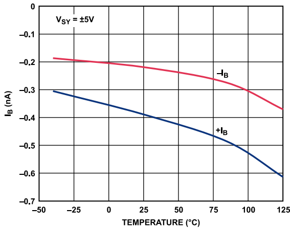
Figure 24. Input Bias Current ( I_B ) vs. Temperature, V_{SY} = \pm 5 V
