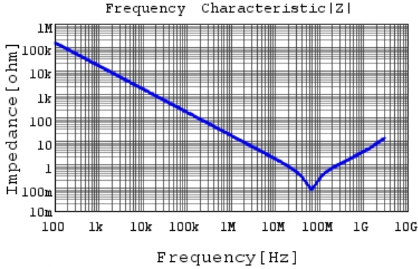
GRM21BR72H103KW09 |Z| DCOV, 25degC
