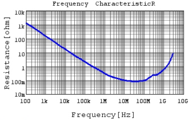
GRM21BR72H103KW09 R DCOV, 25degC
