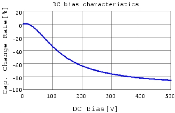
GRM21BR72H103KW09 C-DC bias capchange, 25.0c
