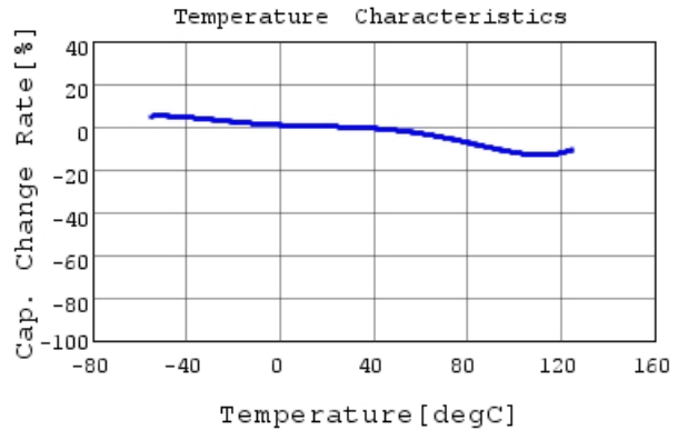
GRM21BR72H103KW09 C-Temp. capchange, DCOV, 1
