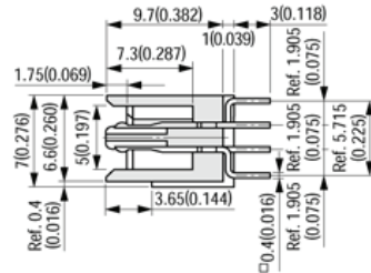
X-X' Cross Section
