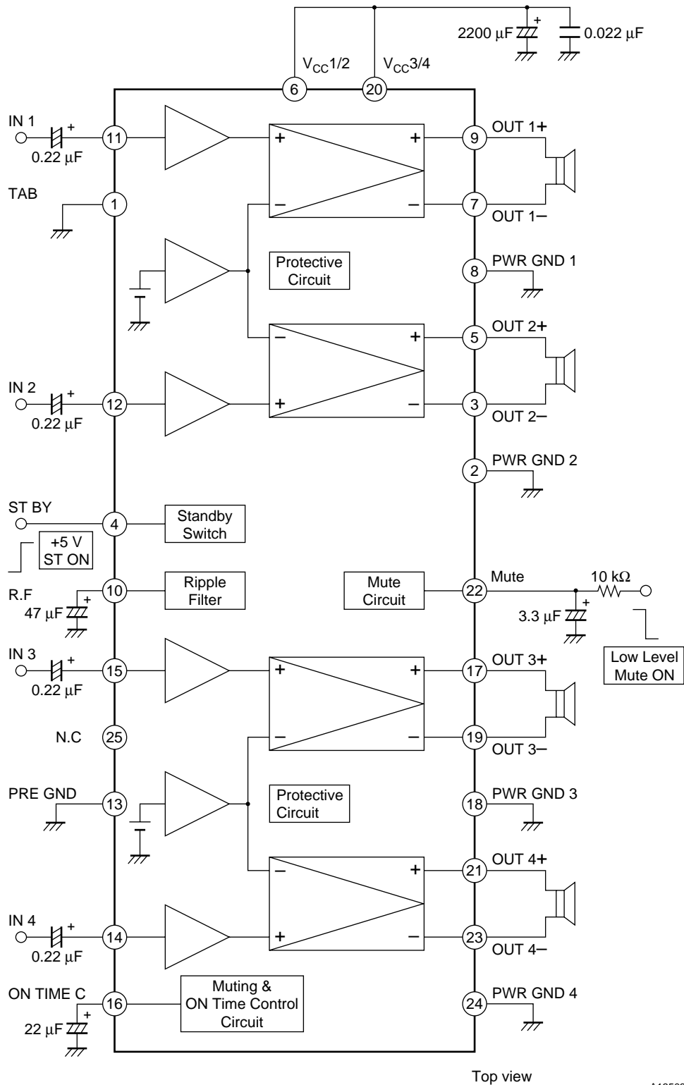
Top view
