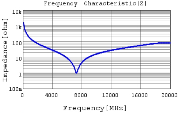
GRM1555C1H1R0BA01 |Z| DCOV, 25degC
