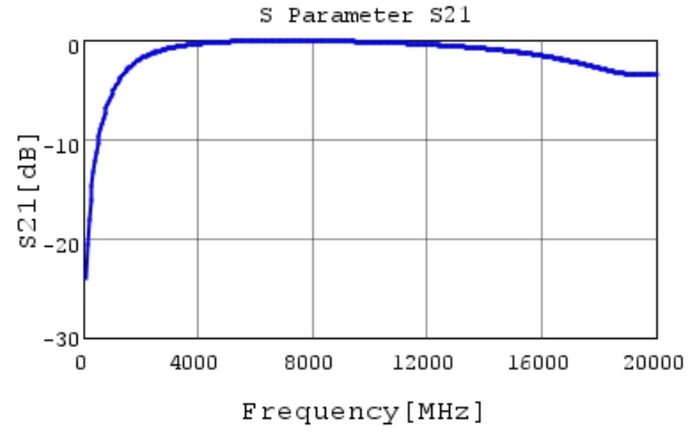
GRM1555C1H1R0BA01 S21 DCOV, 25degC
