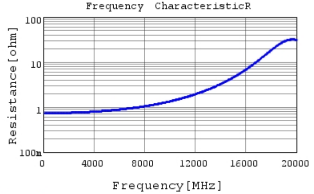
GRM1555C1H1R0BA01 R DCOV, 25degC
